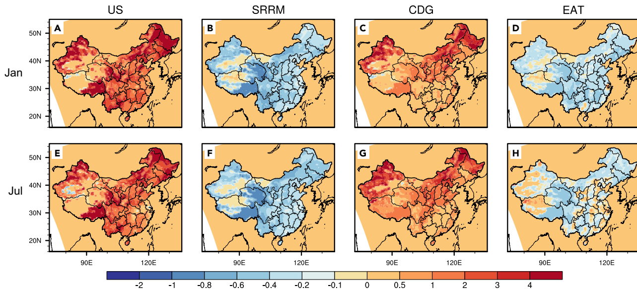
Figure 2. Changes in \text{NH}_3 emissions in potential dietary scenarios relative to Baseline diet \text{NH}_3 emissions in January and July of 2012
