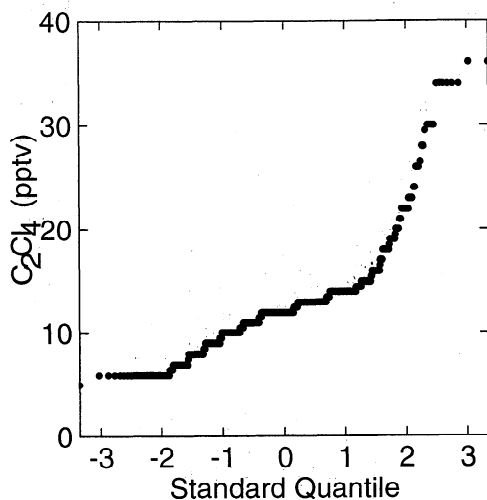
Figure 7. Probability distribution function of C_2Cl_4 concentrations in ABLE 3B.
