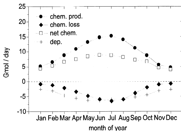
Figure 6. Seasonal variations of chemical production (chem. prod.), chemical loss (chem. loss), net chemical production (net chem.) and dry deposition (dep.) of ozone in the boundary layer (0-2.1 km) of East Asia. Units are Gmol/day.
